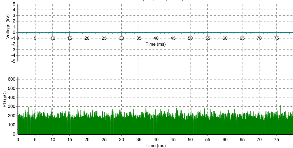
L2@0.0 kV Test 1 PD level: 314 pC ; frequency: - Hz
