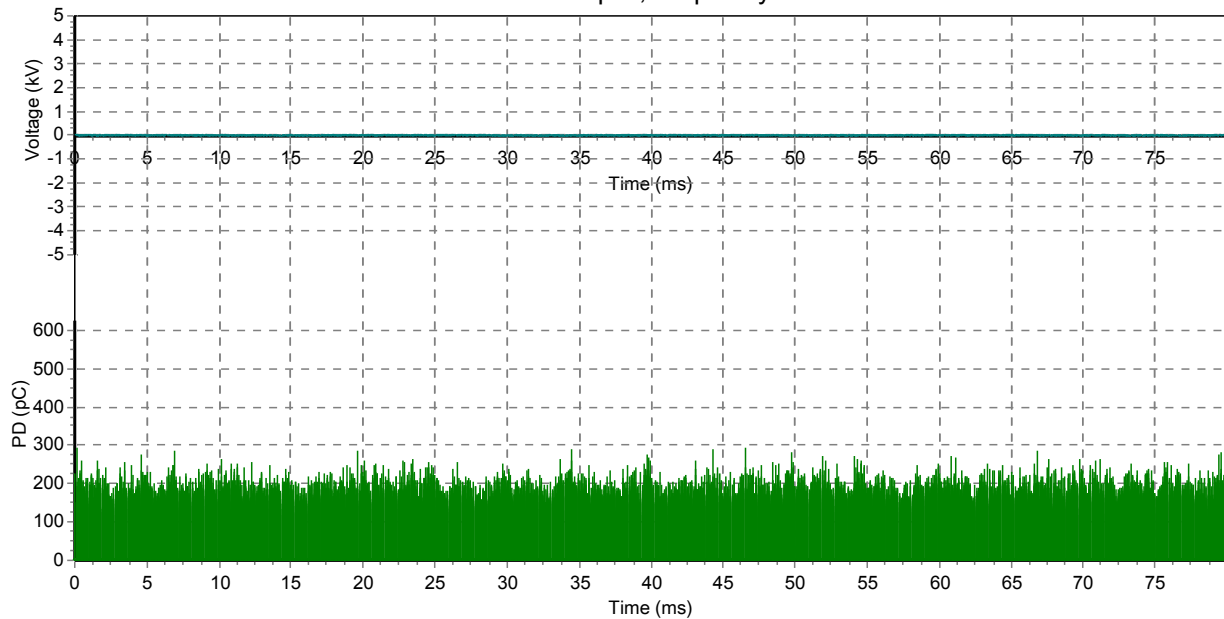
L1 @0.0 kV Test 1 PD level: 292 pC ; frequency: - Hz
