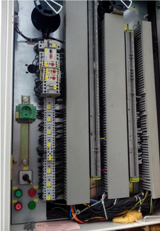
Lampiran 2. Wiring Control Box PMT.
