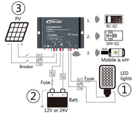
Figure 2 Wiring
